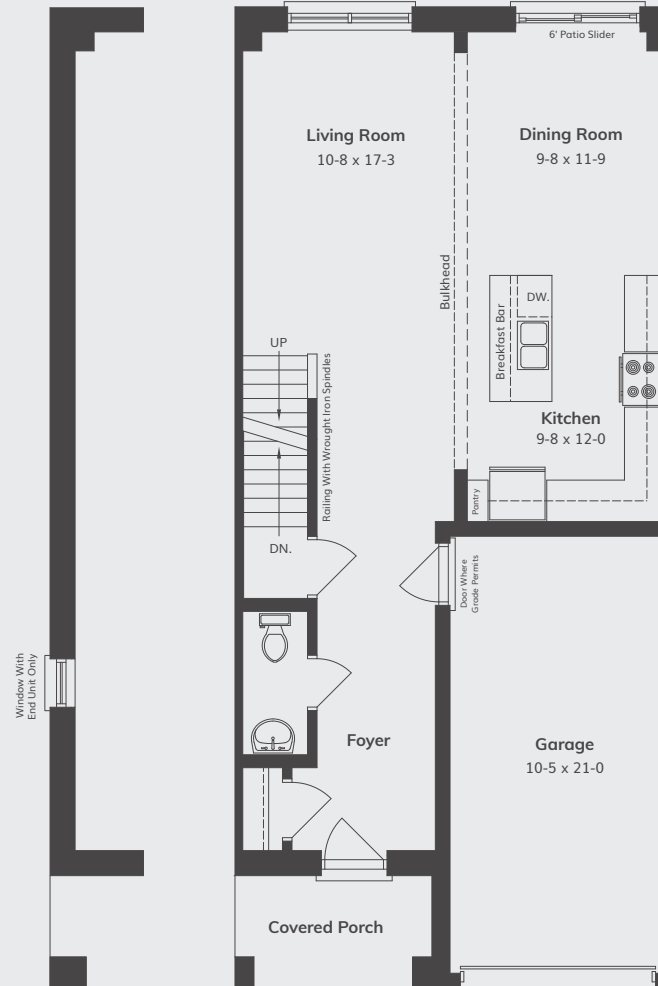
Main Floor End Unit Elevation A & B
